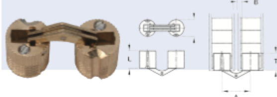
USY SCHARNIER 180°
